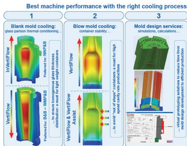
Cooling overview.
