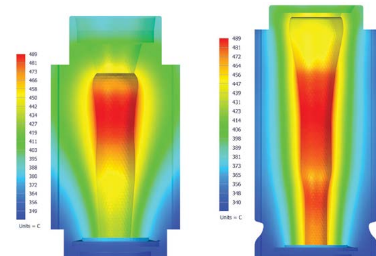
Cooling overview.
